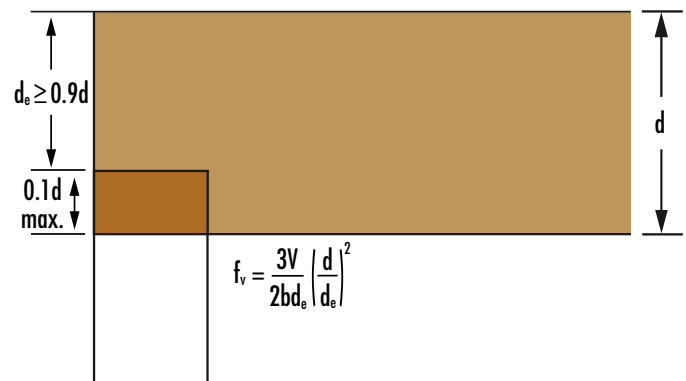
Tension-side Notch
