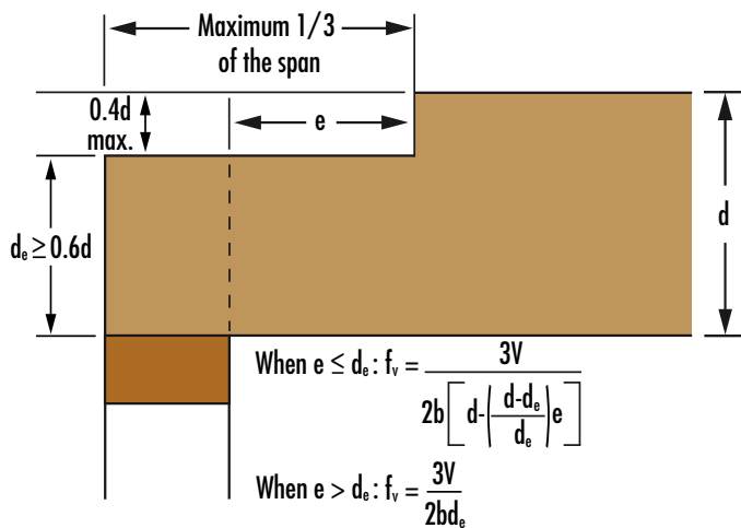
Compression-side Notch
